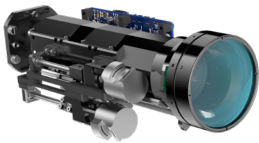
SWIR 25-250mm f/5.5, f/4.0 > 26km detection range
