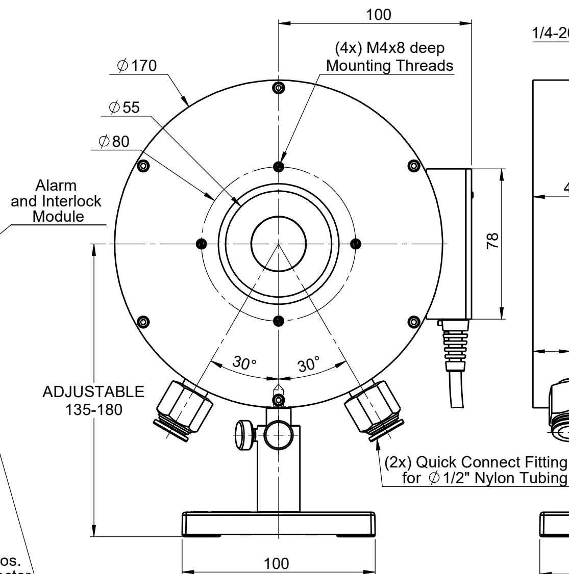
Front Side
