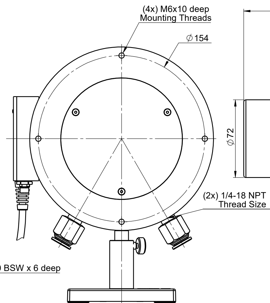
Rear Side
