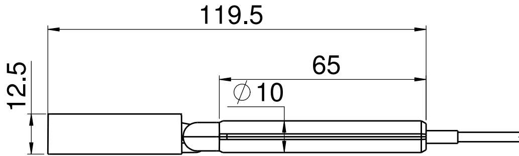
VIEW A
