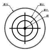
16K-W Scatter Shield Cover
