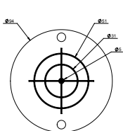
16K-W Protective Cover
