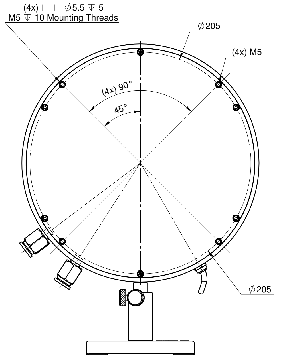
Back Side
