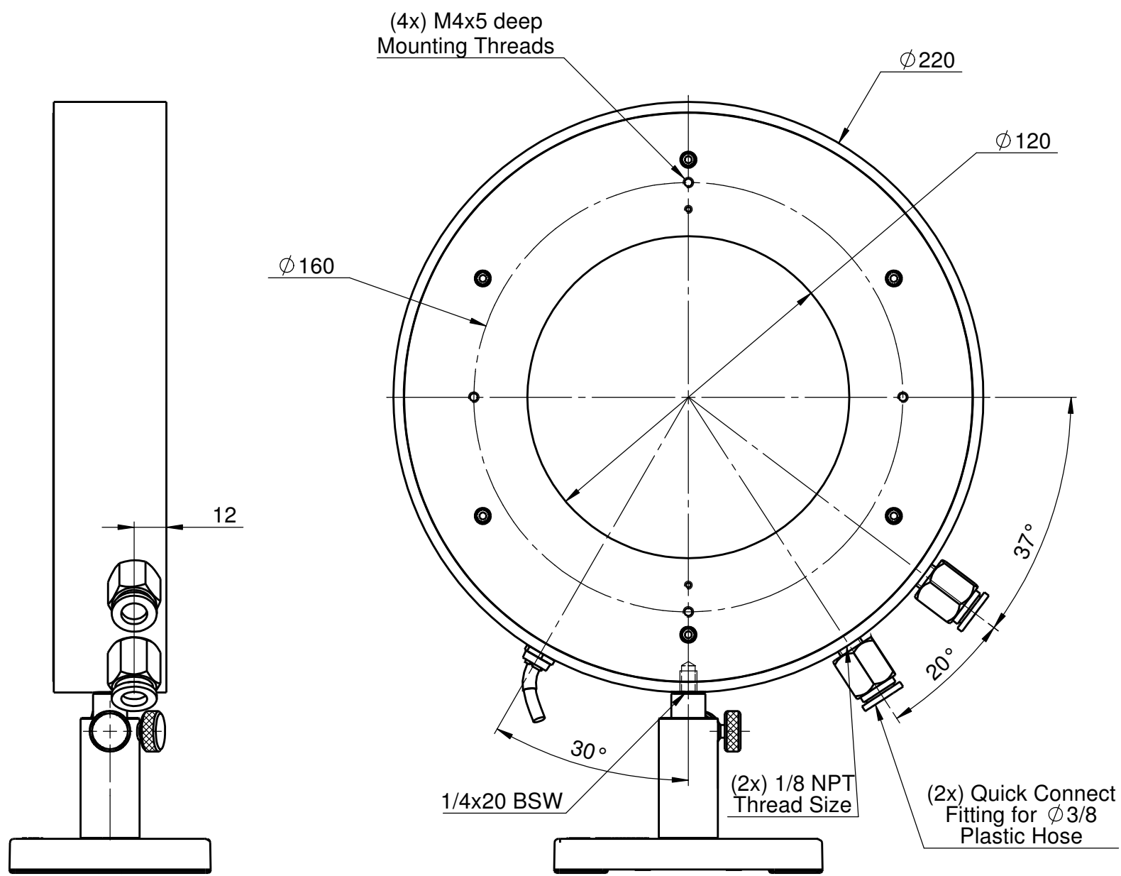
Front Side
