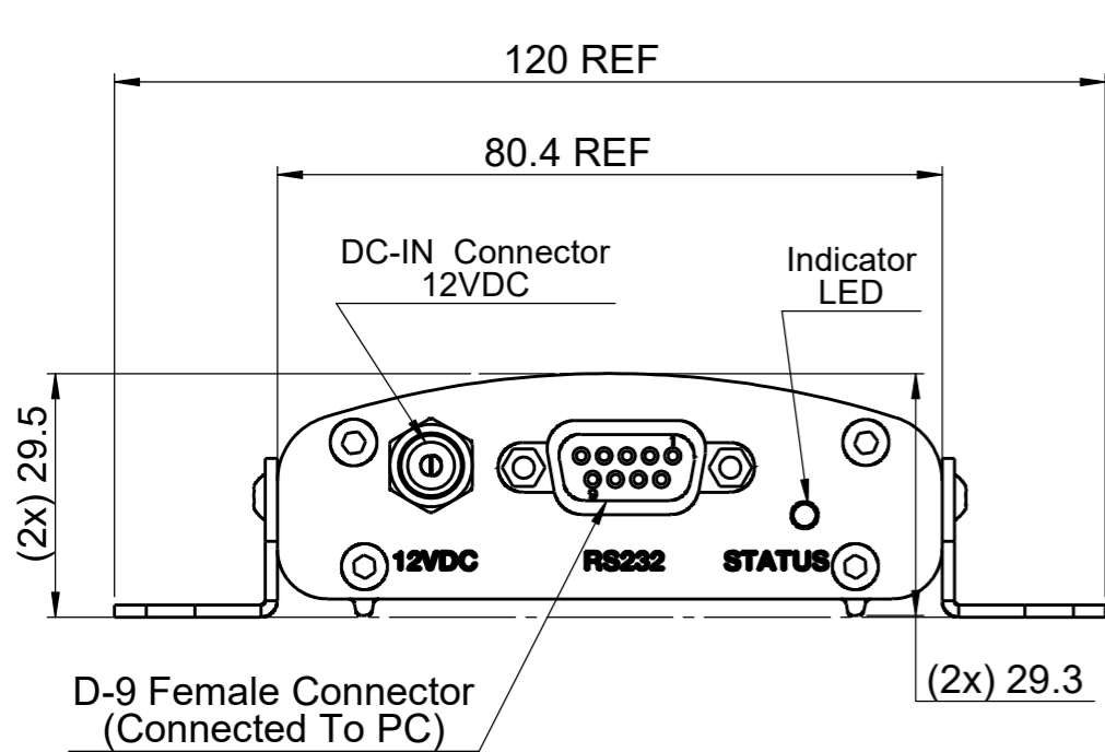
Rear View
