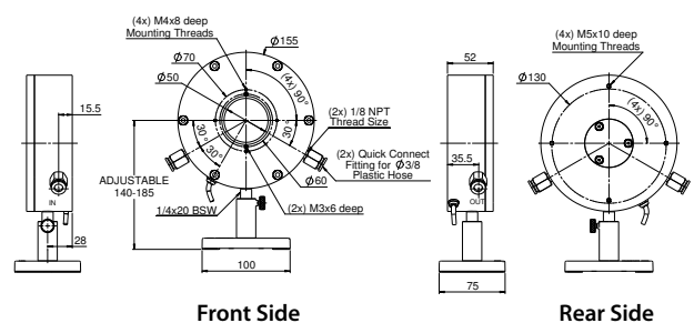
5000WP-LP2-50
