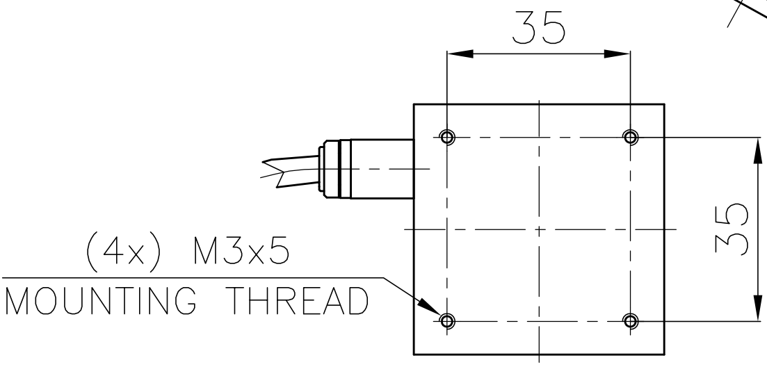
VIEW A
