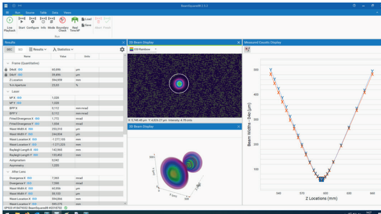
Fig. 5: Measurements taken with the MKS Ophir BeamSquared beam propagation analyzer prove the high quality of the Yucca 100-343 laser under test.
